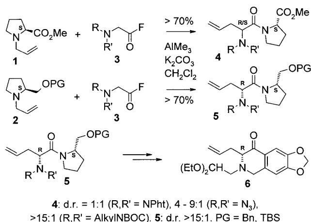
Scheme 1. Overview: diastereoselective aza-Claisen rearrangements of N -allylamines 1 and 2 .
