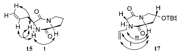
Figure 1. NOESY analyses of piperazinediones 15 and 17 . Significant correlations are marked with arrows, pivotal effects are marked with “!”.
