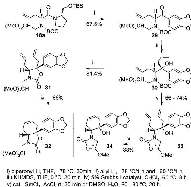
Scheme 7. Syntheses of optically active cyclohexenes.
