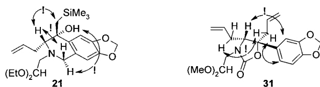
Figure 3. NOESY Analyses of allyl adducts 21 and 31 . Significant correlations are marked with arrows, pivotal effects are marked with “!”.
