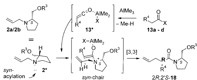
Figure 2. Stereochemical rationalization of the auxiliary controlled aza-Claisen rearrangement: working hypothesis.
